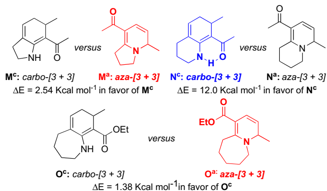
Figure 4. Energetic differences in the annulation products.
