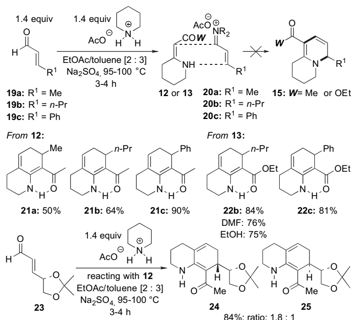
Scheme 5. Unexpected formation of hexahydroquinolines.
