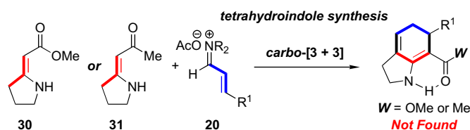
Figure 3. A possible synthesis of tetrahydroindoles.
