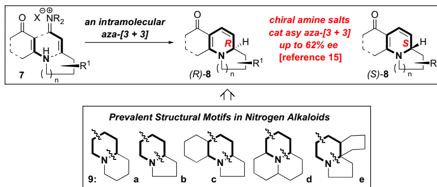
Scheme 2. An intramolecular aza-[3+3] annulation.
