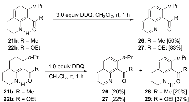
Scheme 7. DDQ aromatization in the quinoline synthesis.
