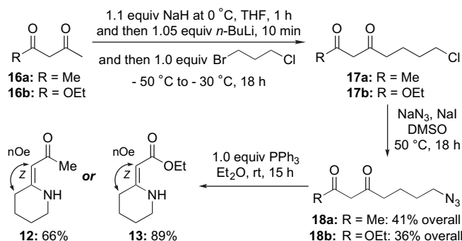
Scheme 4. Syntheses of exo -cyclic vinylogous amide and urethane.
