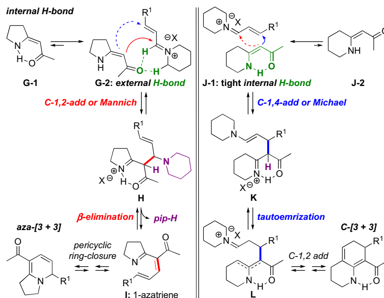
Scheme 8. C-1,2 addition versus C-1,4-addition.
