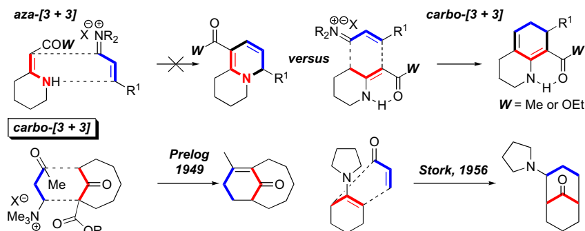
Figure 2. Aza-[3+3] versus carbo-[3+3] annulation.
