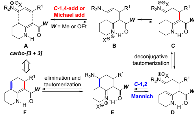
Scheme 6. A proposed pathway for the hexahydroquinoline formation.
