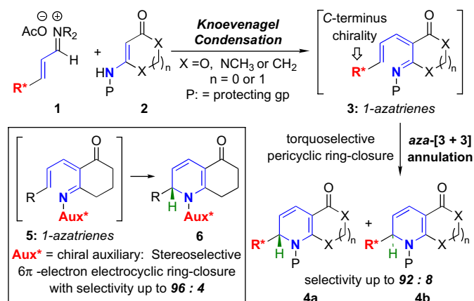
Scheme 1. An aza-[3+3] annulation.
