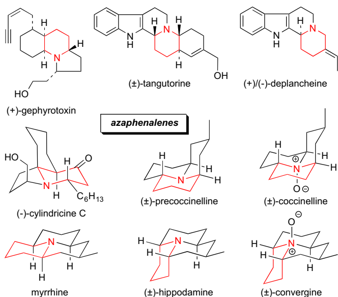
Figure 1. Alkaloids synthesized via intramolecular aza-[3+3].
