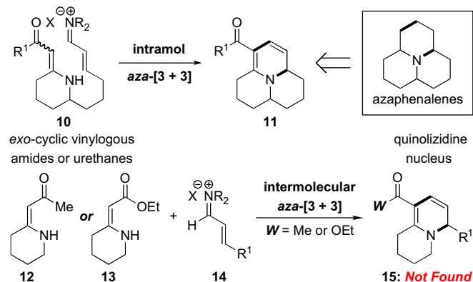
Scheme 3. An aza-[3+3] pathway to azaphenalenes and quinolizidines.
